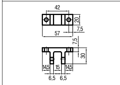
Aluminium back bracket part No. 35697P
