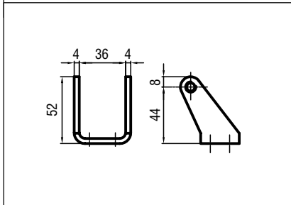
Steel end bracket included (No accessories included in Ulysses RWA version)
